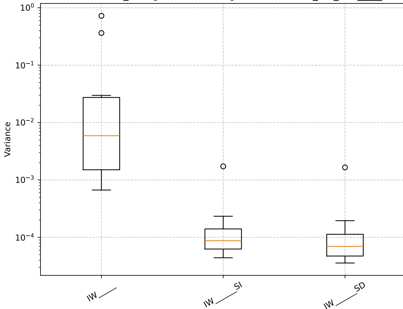
Q=2.22, len_rolling=100: Shrinkage Box Plot - min_var_, IW_____
