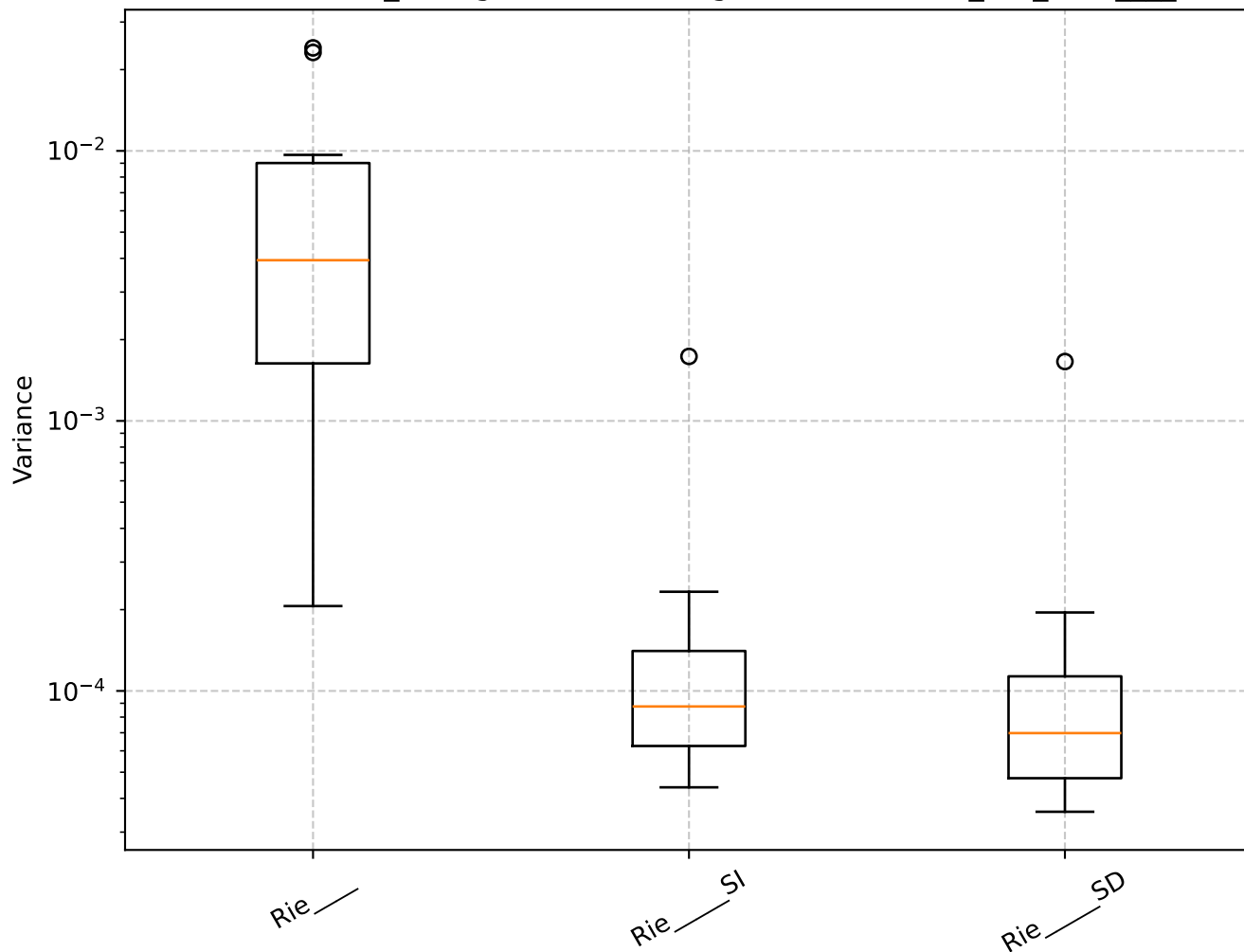
Q=2.35, len_rolling=100: Shrinkage Box Plot - min_var_, Rie____
