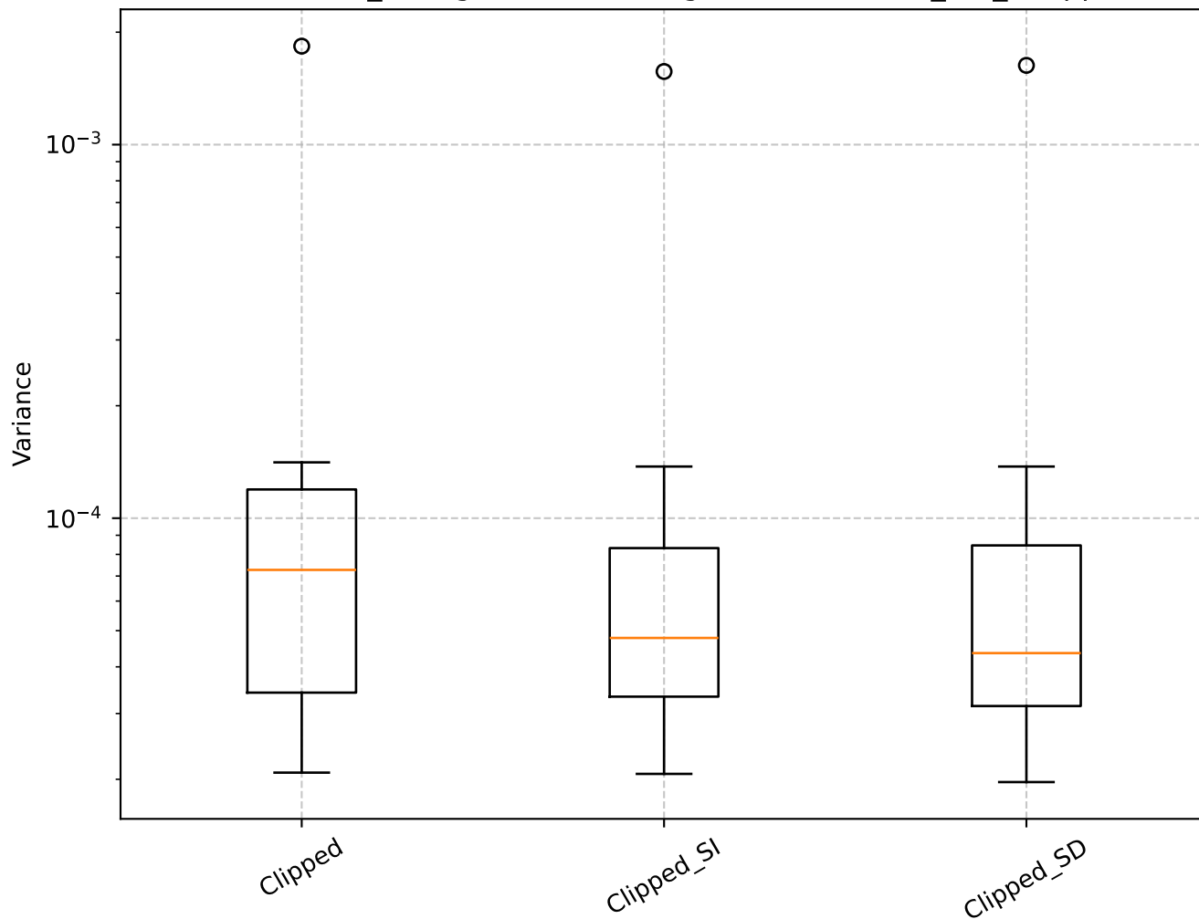
Q=2.50, len_rolling=100: Shrinkage Box Plot - min_var_, Clipped
