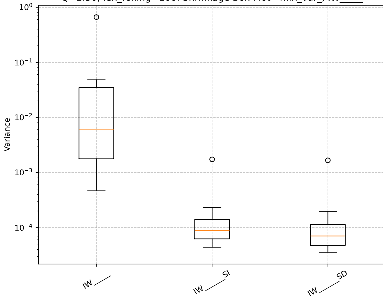
Q=2.50, len_rolling=100: Shrinkage Box Plot - min_var_, IW_____
