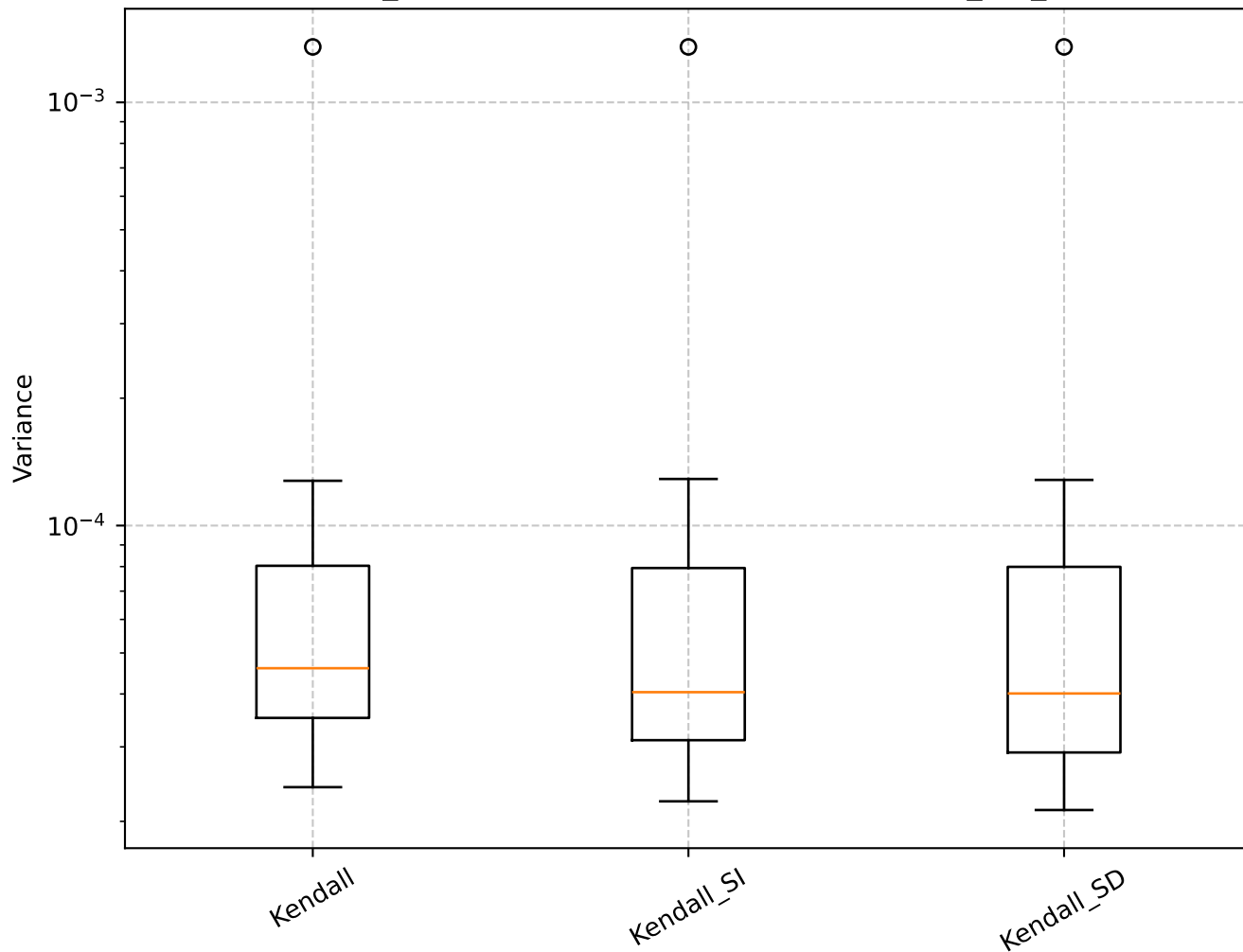
Q=2.50, len_rolling=100: Shrinkage Box Plot - min_var_, Kendall
