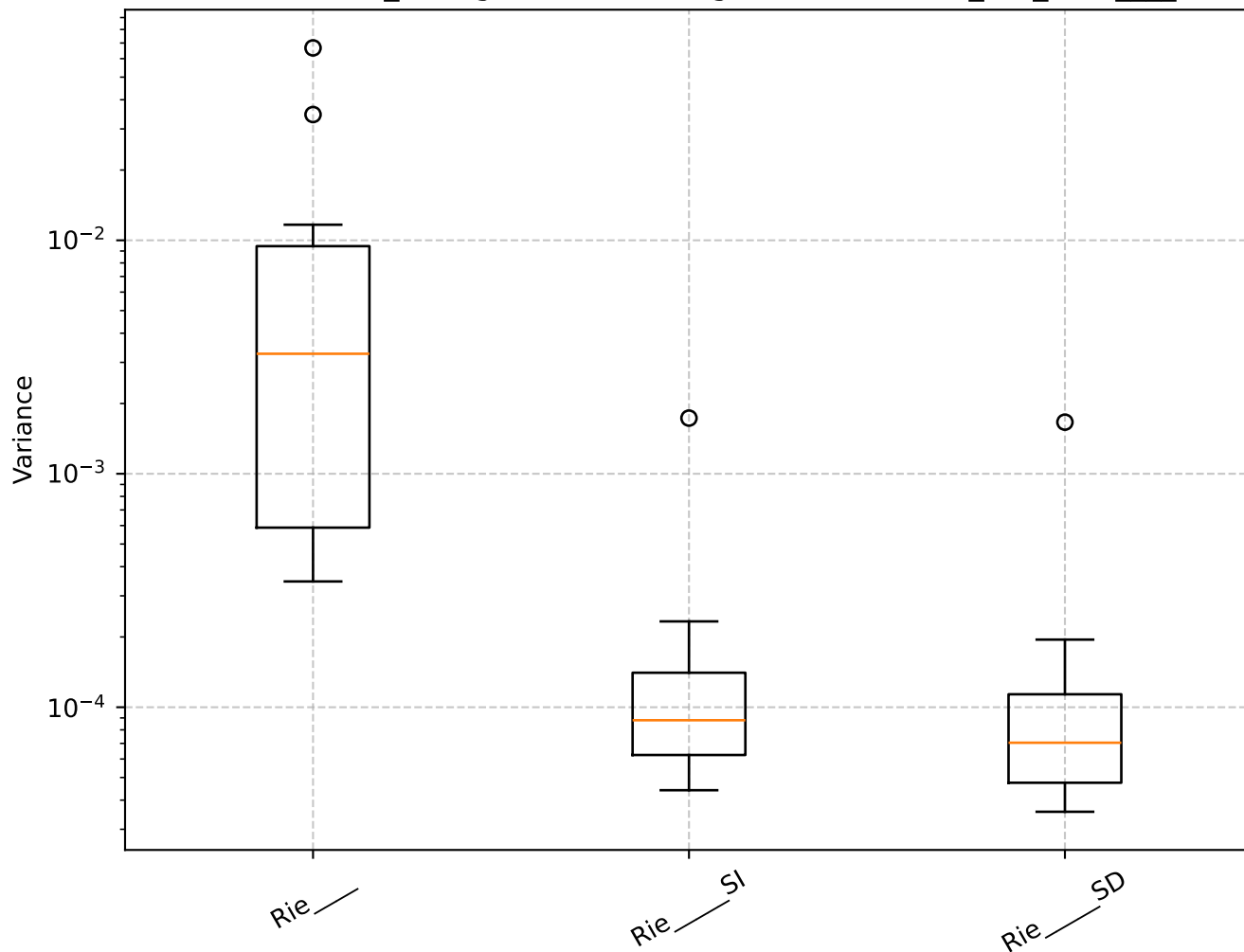
Q=2.50, len_rolling=100: Shrinkage Box Plot - min_var_, Rie____
