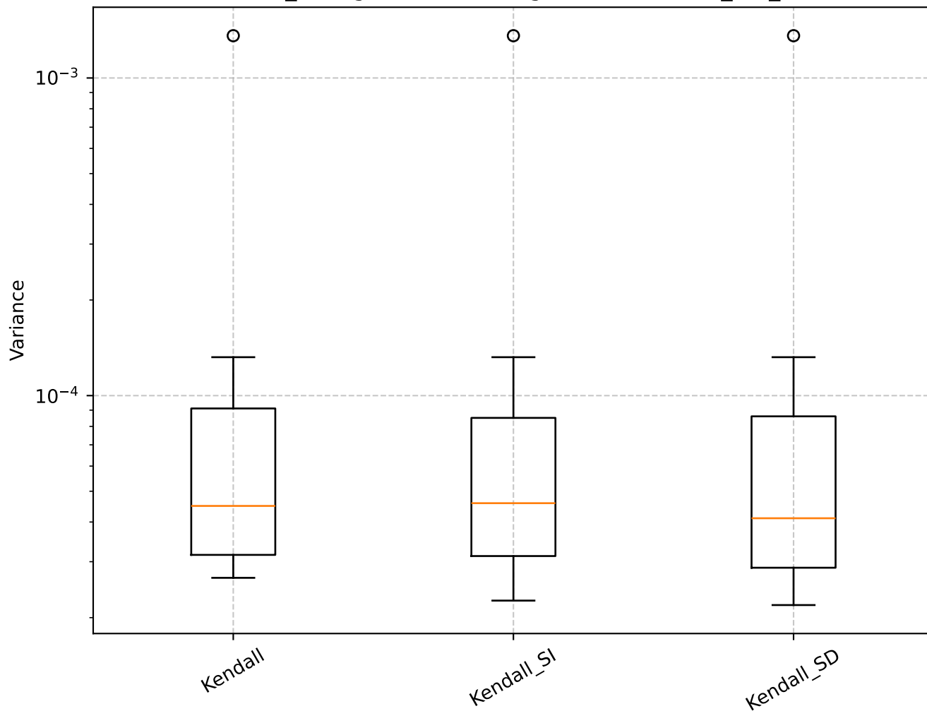
Q=3.10, len_rolling=100: Shrinkage Box Plot - min_var_, Kendall
