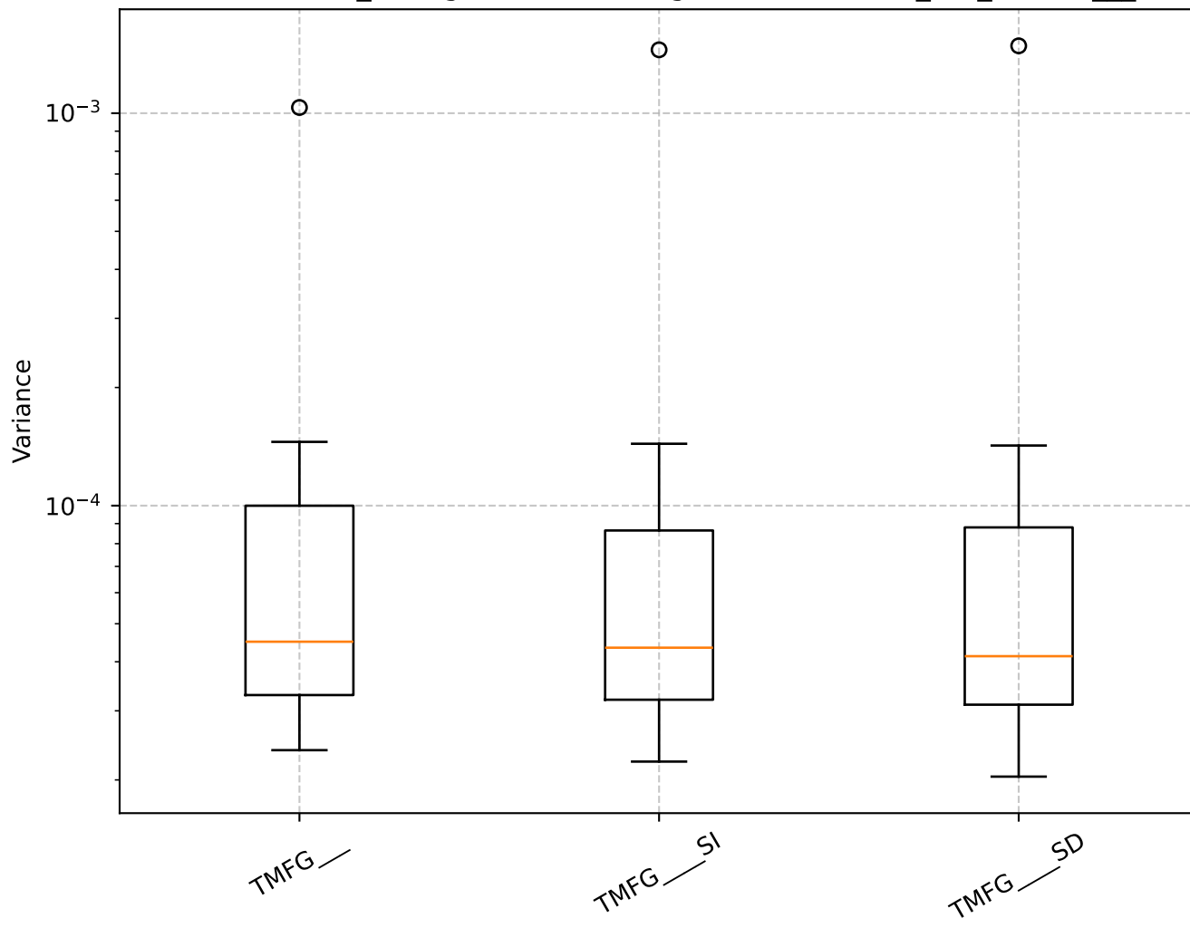
Q=3.10, len_rolling=100: Shrinkage Box Plot - min_var_, TMFG__
