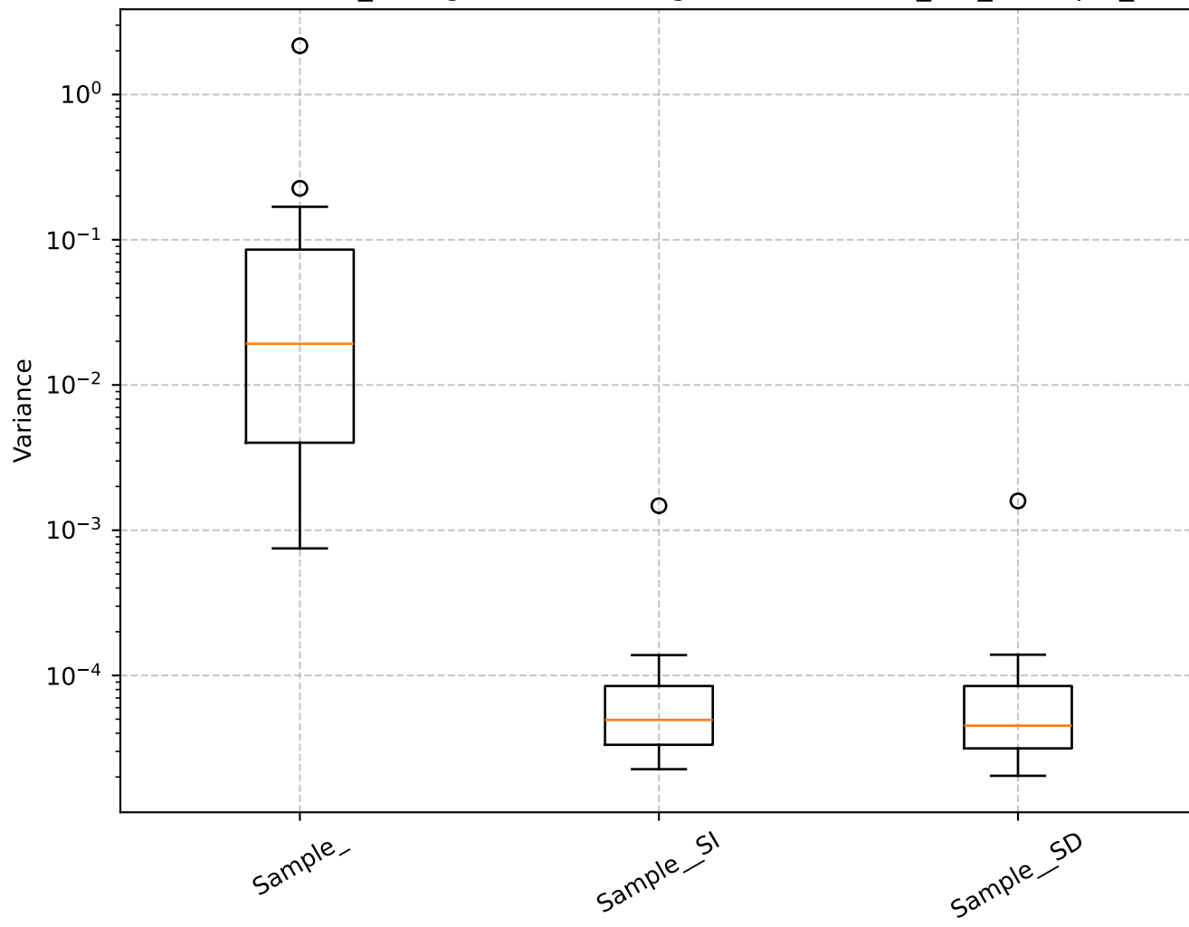
Q=4.00, len_rolling=100: Shrinkage Box Plot - min_var_, Sample_
