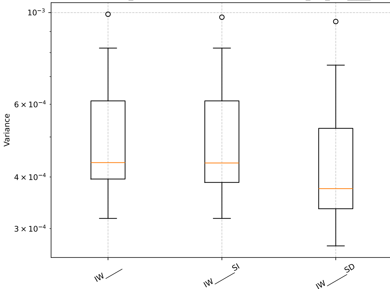
Q=0.50, len_rolling=100: Shrinkage Box Plot - min_var_, IW_____
