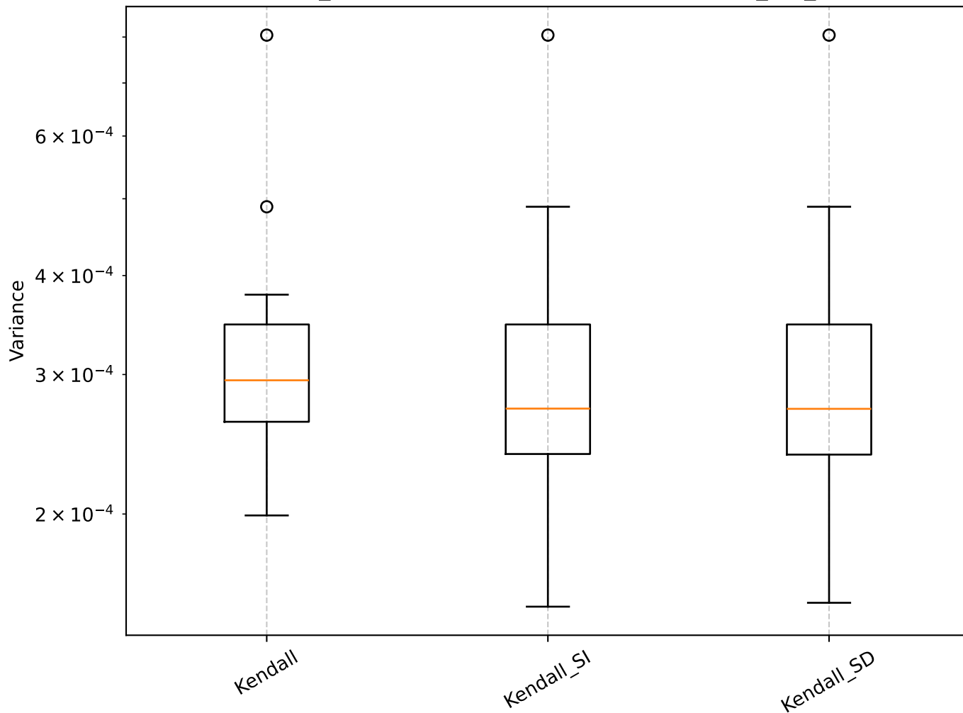
Q=0.51, len_rolling=100: Shrinkage Box Plot - min_var_, Kendall
