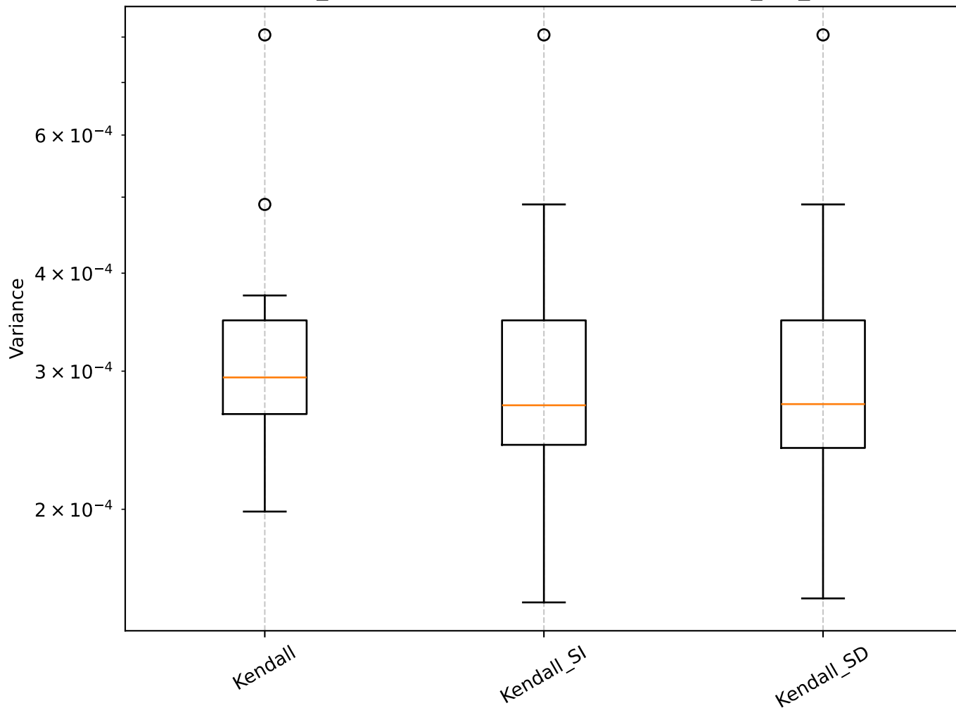
Q=0.52, len_rolling=100: Shrinkage Box Plot - min_var_, Kendall
