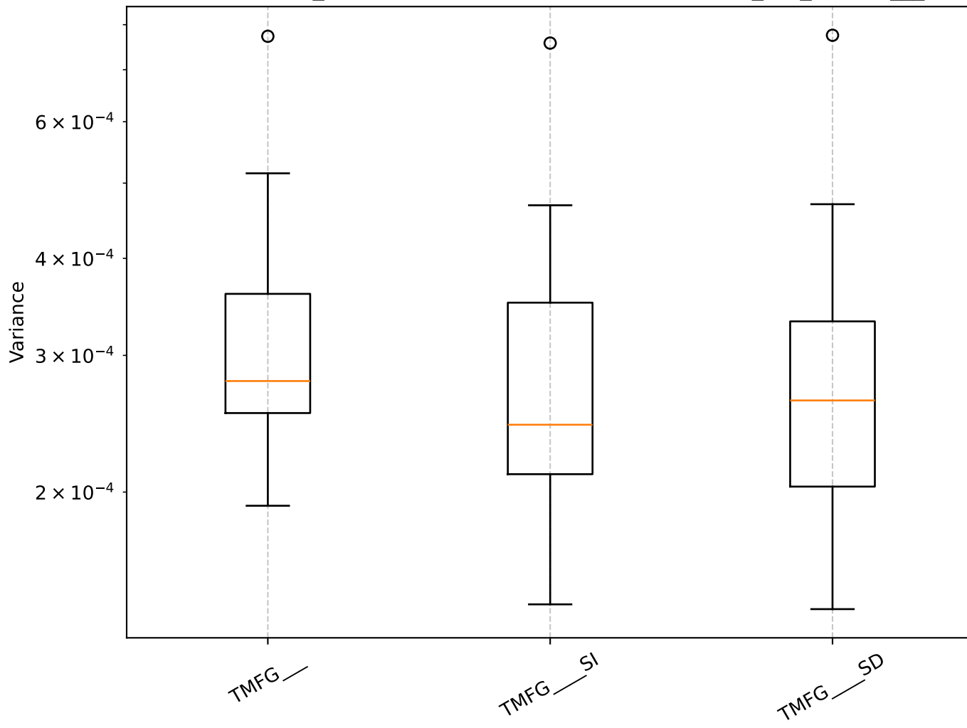
Q=0.52, len_rolling=100: Shrinkage Box Plot - min_var_, TMFG__
