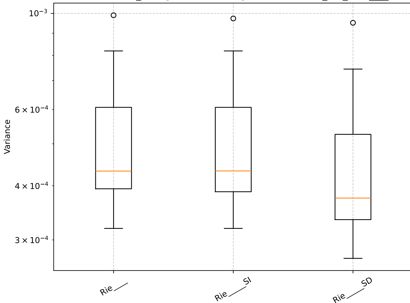
Q=0.53, len_rolling=100: Shrinkage Box Plot - min_var_, Rie__
