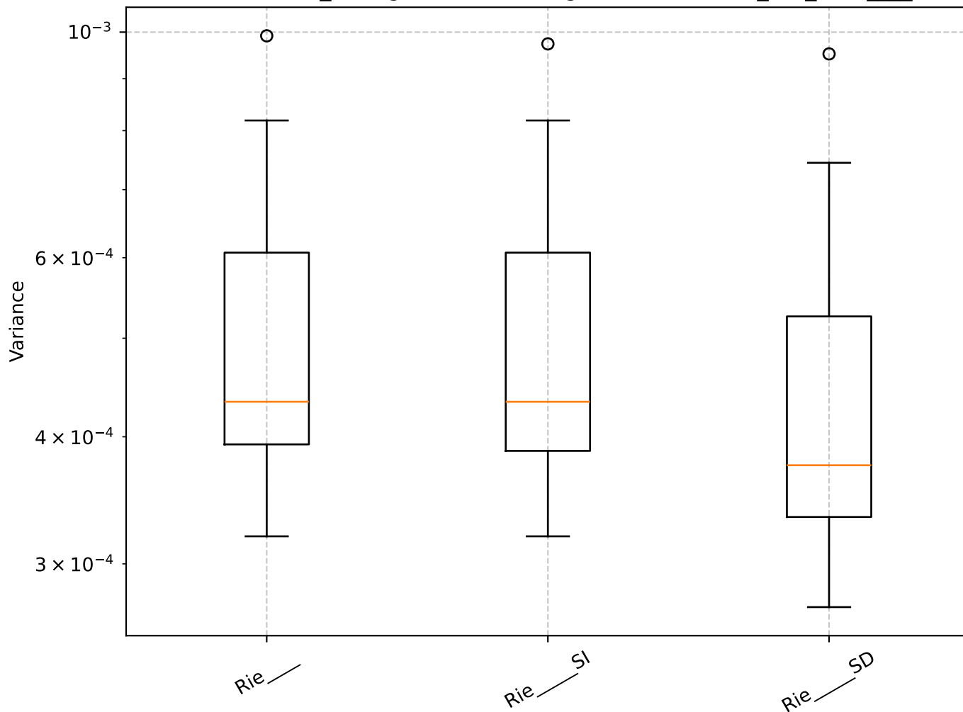
Q=0.54, len_rolling=100: Shrinkage Box Plot - min_var_, Rie__
