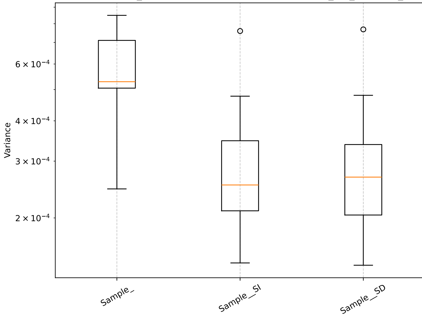
Q=0.54, len_rolling=100: Shrinkage Box Plot - min_var_, Sample_
