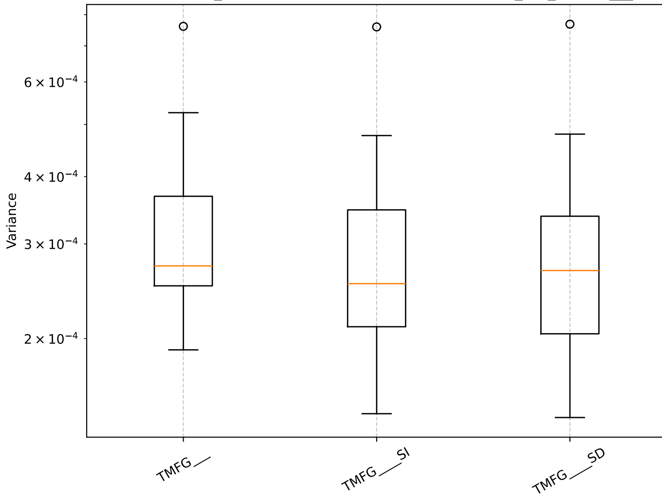
Q=0.54, len_rolling=100: Shrinkage Box Plot - min_var_, TMFG__
