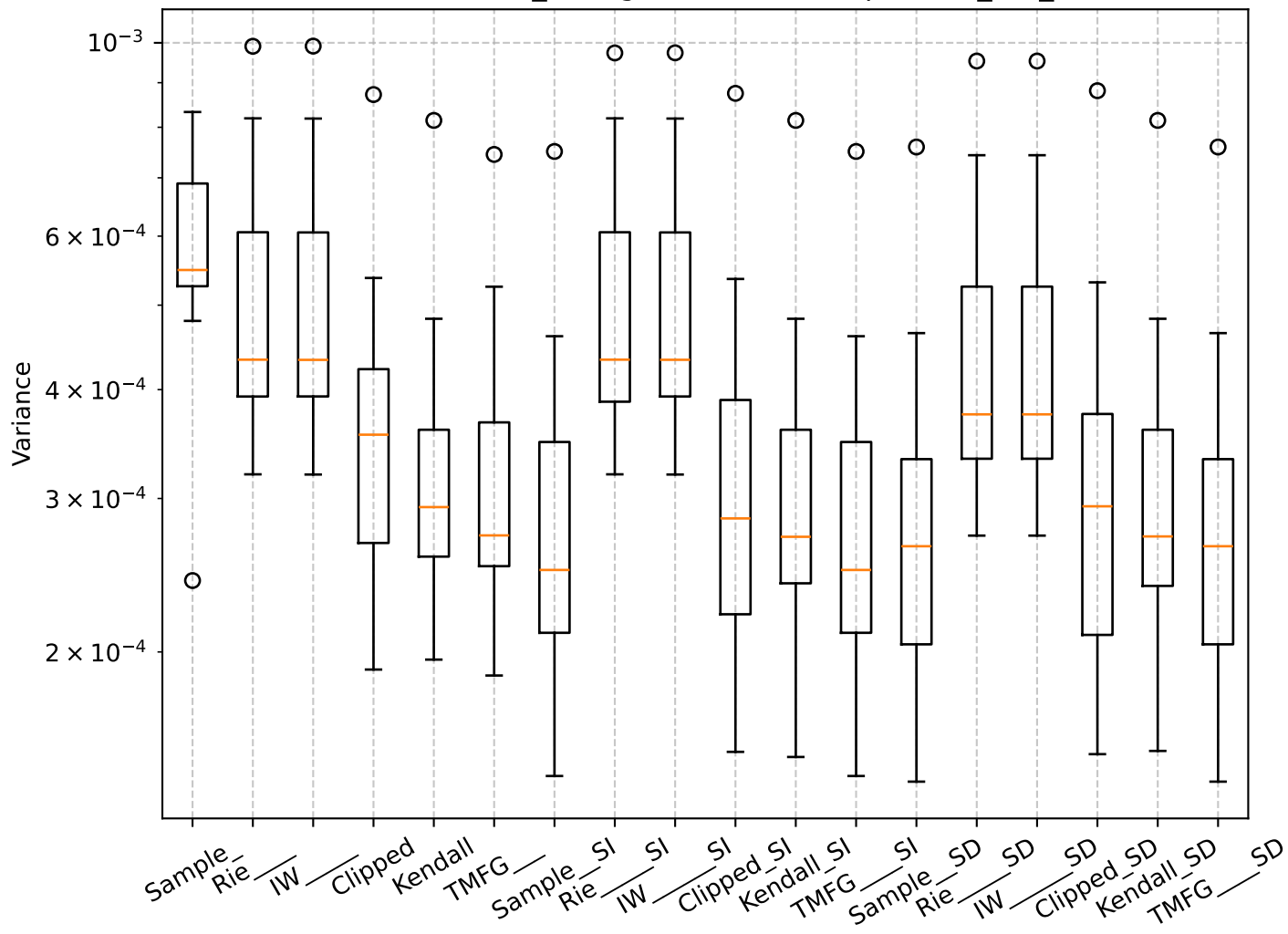
Q=0.55, len_rolling=100: Box Plot per min_var_
