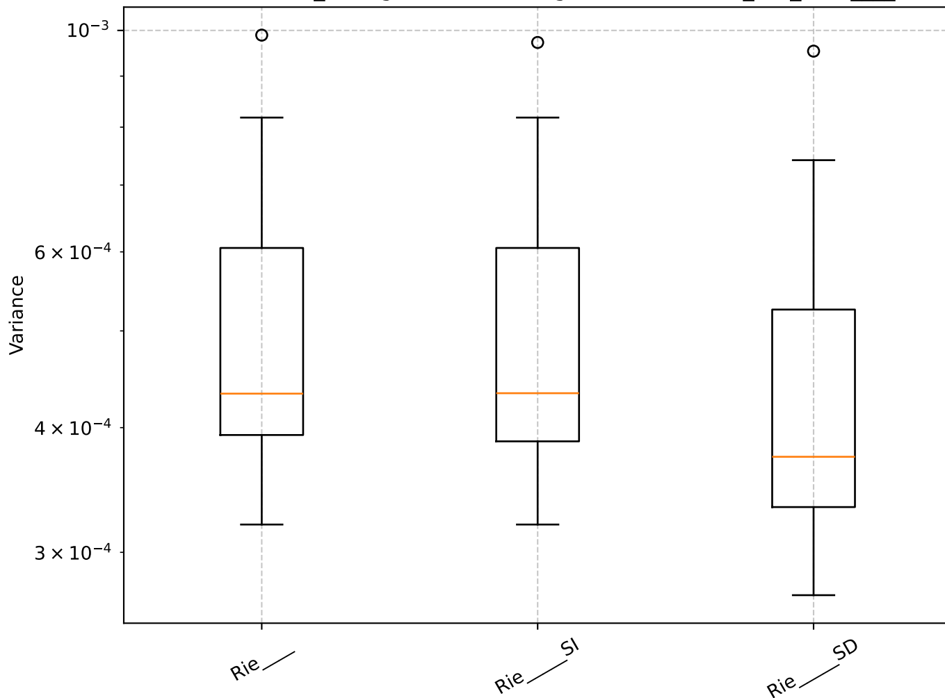
Q=0.56, len_rolling=100: Shrinkage Box Plot - min_var_, Rie__
