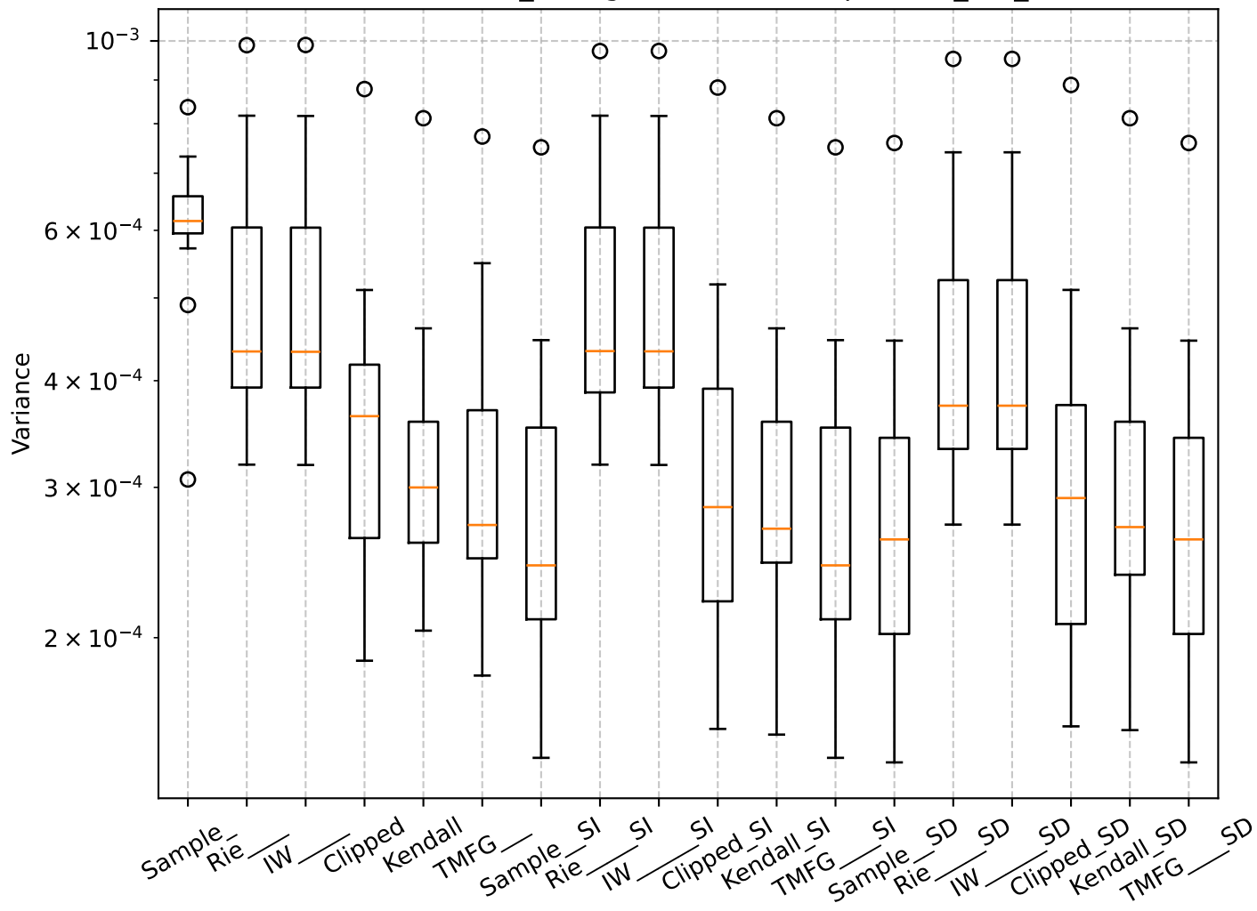
Q=0.57, len_rolling=100: Box Plot per min_var_
