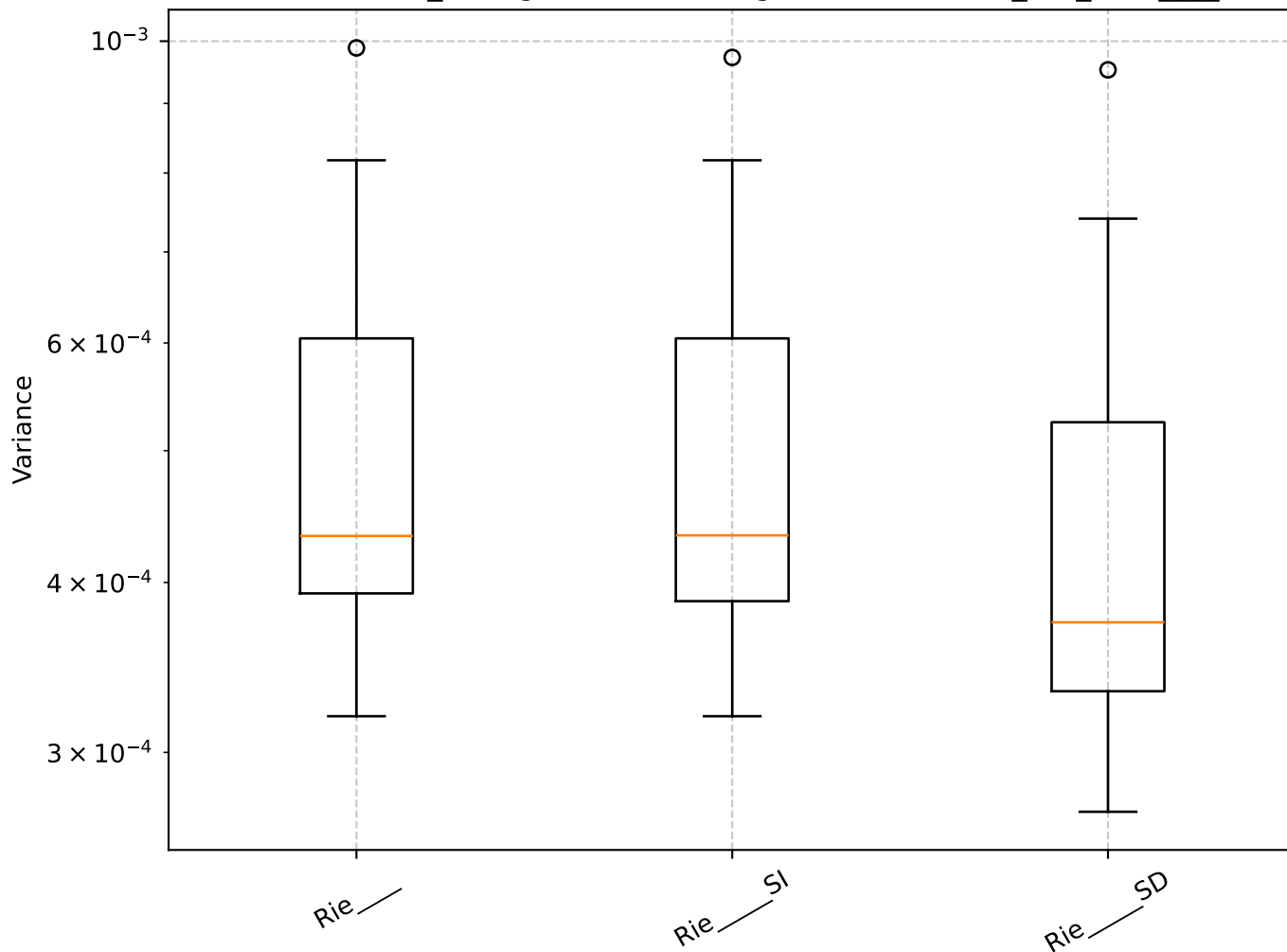
Q=0.57, len_rolling=100: Shrinkage Box Plot - min_var_, Rie__
