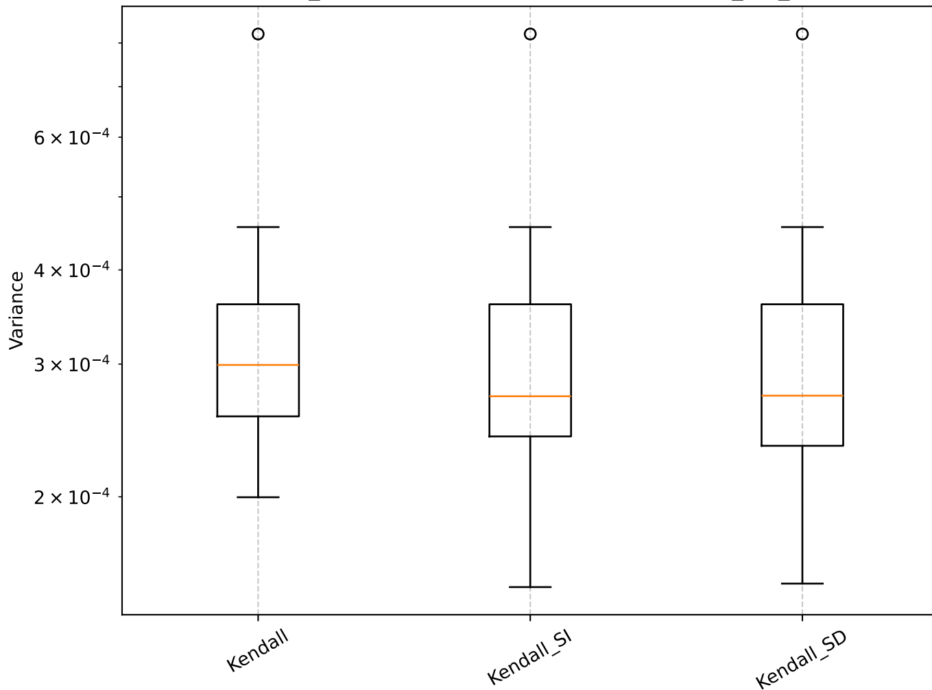
Q=0.59, len_rolling=100: Shrinkage Box Plot - min_var_, Kendall
