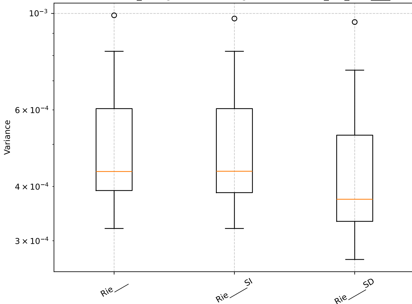
Q=0.59, len_rolling=100: Shrinkage Box Plot - min_var_, Rie__
