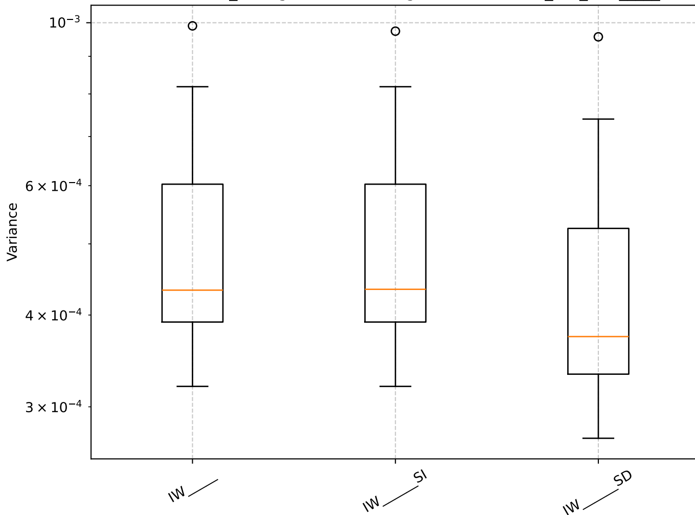
Q=0.60, len_rolling=100: Shrinkage Box Plot - min_var_, IW_____
