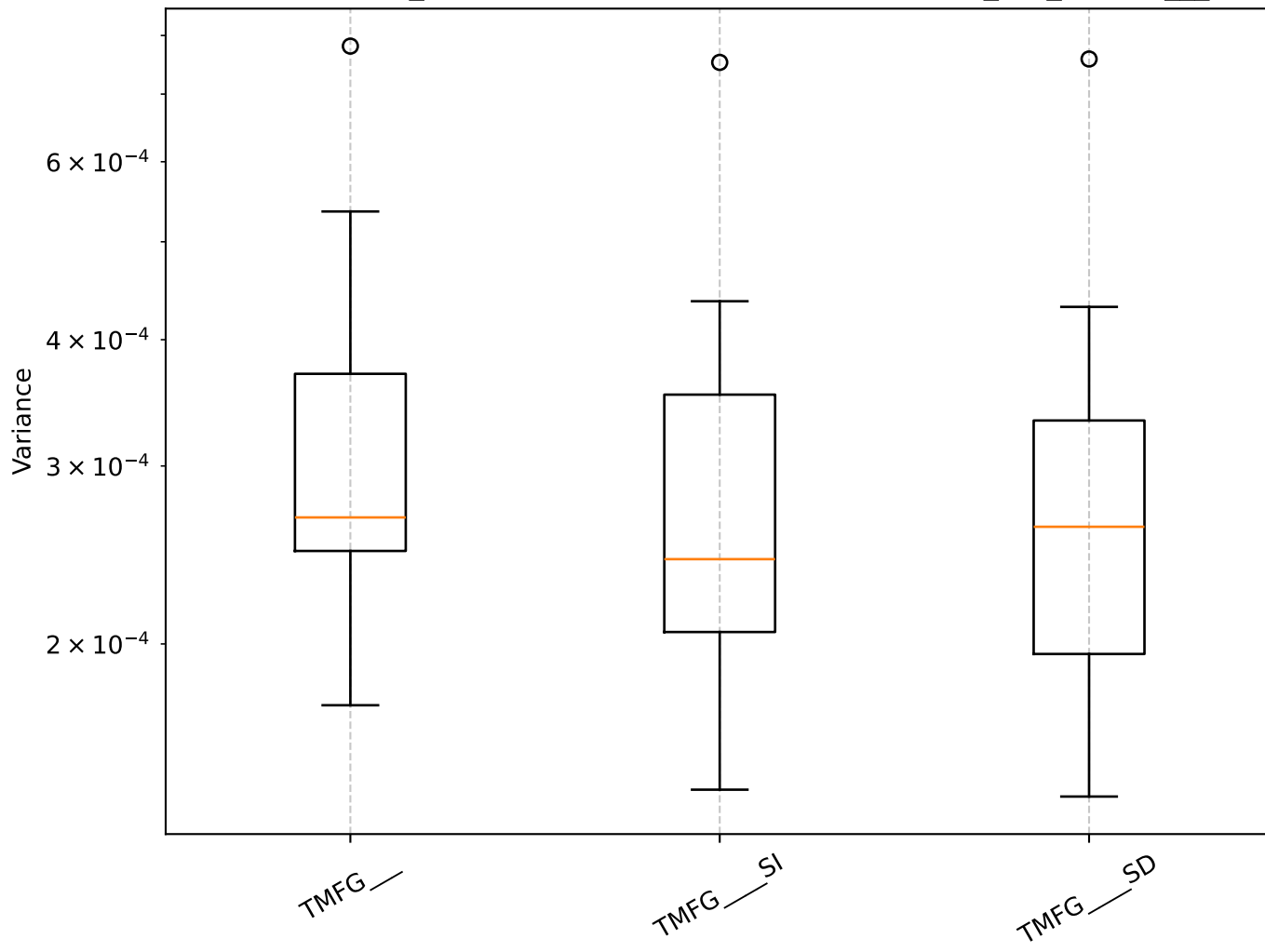
Q=0.60, len_rolling=100: Shrinkage Box Plot - min_var_, TMFG__
