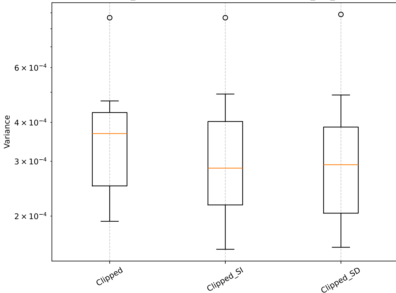
Q=0.61, len_rolling=100: Shrinkage Box Plot - min_var_, Clipped
