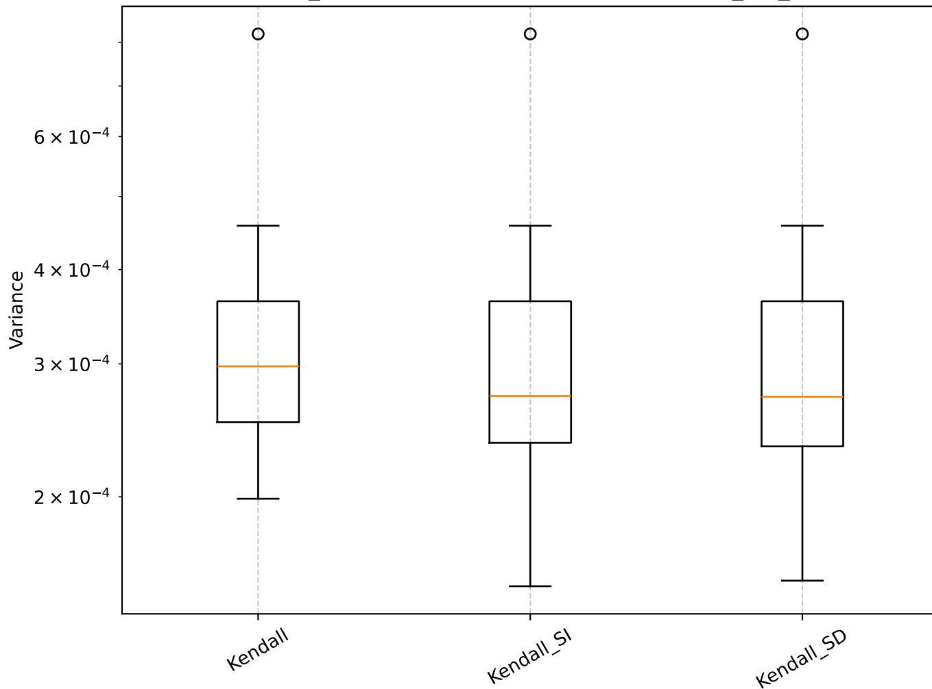
Q=0.61, len_rolling=100: Shrinkage Box Plot - min_var_, Kendall
