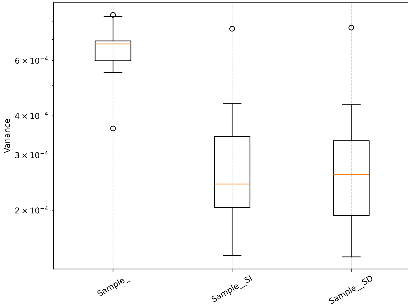
Q=0.61, len_rolling=100: Shrinkage Box Plot - min_var_, Sample_
