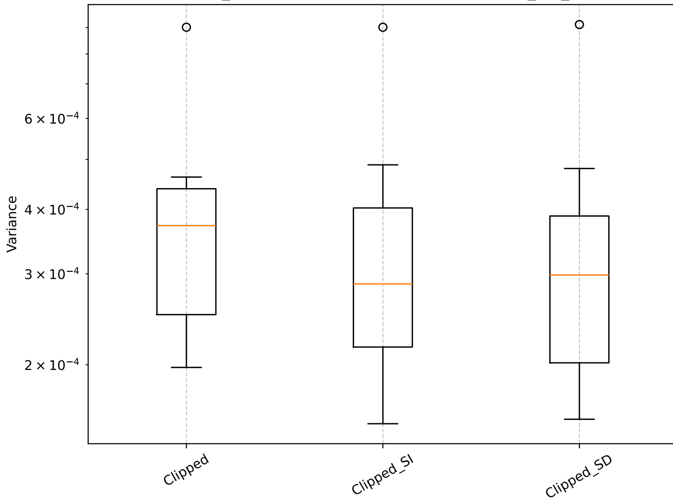
Q=0.62, len_rolling=100: Shrinkage Box Plot - min_var_, Clipped
