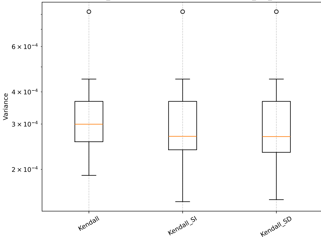
Q=0.63, len_rolling=100: Shrinkage Box Plot - min_var_, Kendall
