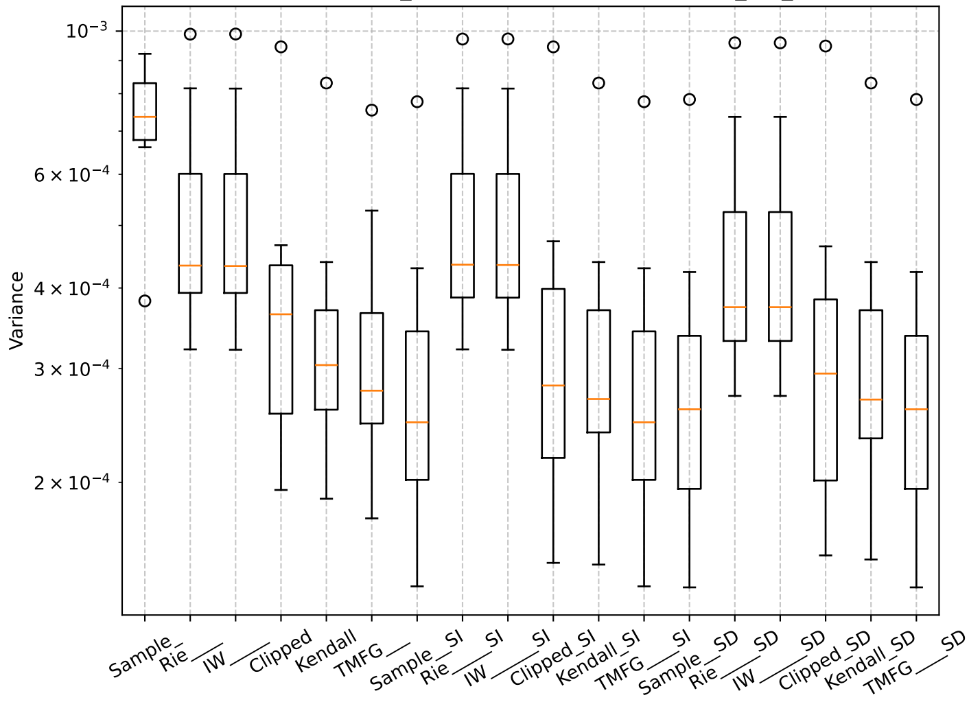
Q=0.65, len_rolling=100: Box Plot per min_var_
