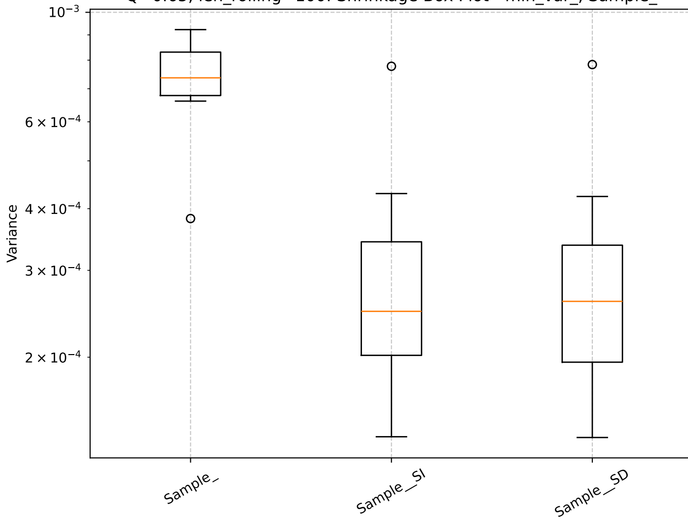
Q=0.65, len_rolling=100: Shrinkage Box Plot - min_var_, Sample_
