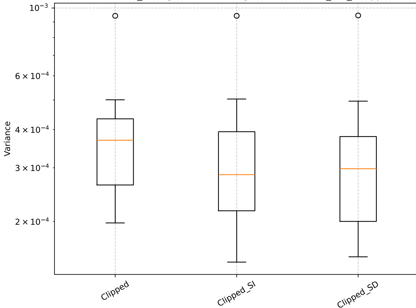
Q=0.66, len_rolling=100: Shrinkage Box Plot - min_var_, Clipped
