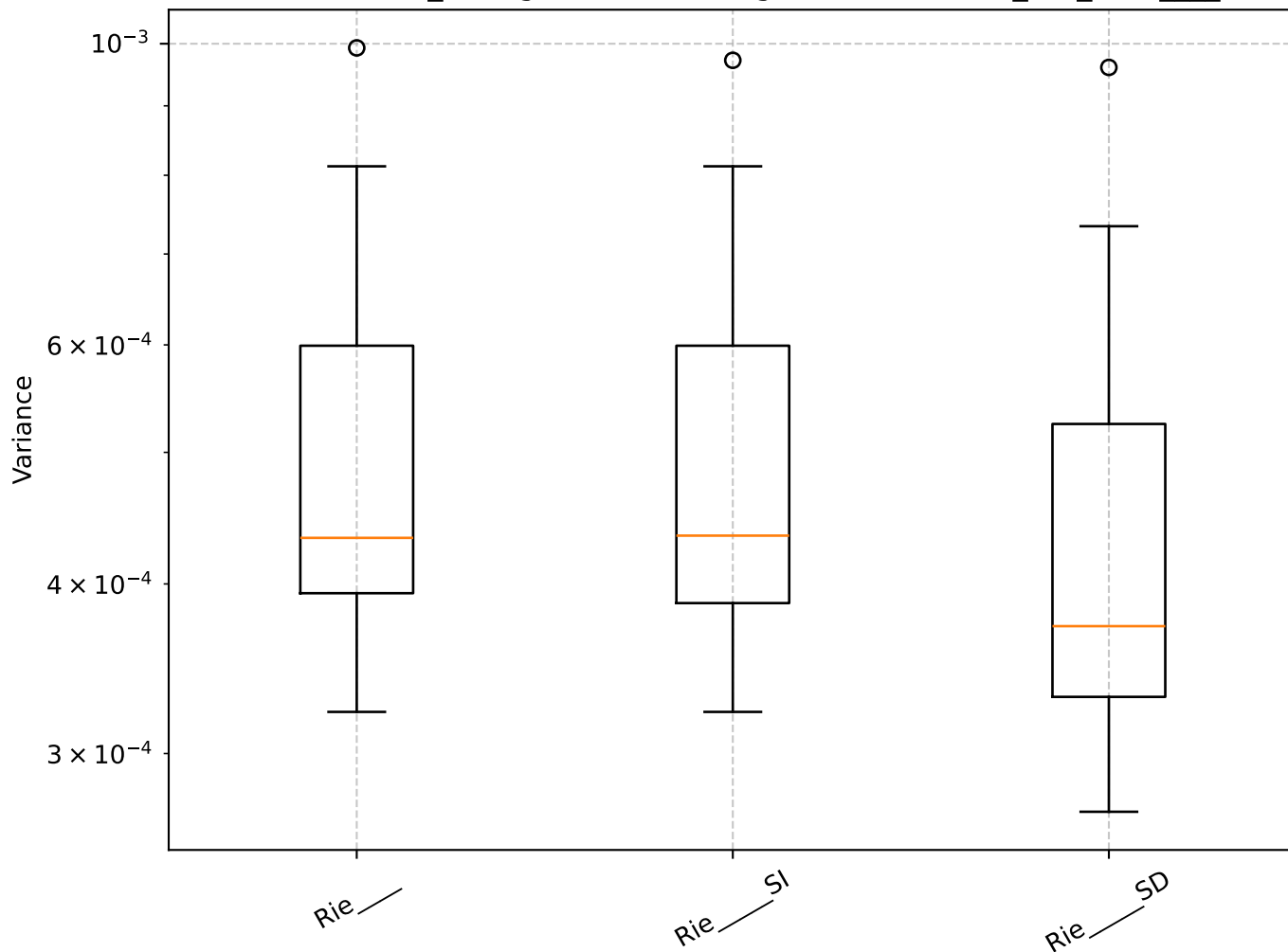
Q=0.69, len_rolling=100: Shrinkage Box Plot - min_var_, Rie__
