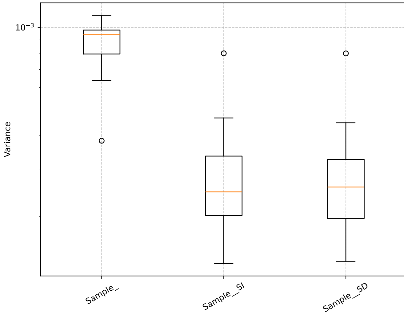
Q=0.69, len_rolling=100: Shrinkage Box Plot - min_var_, Sample_
