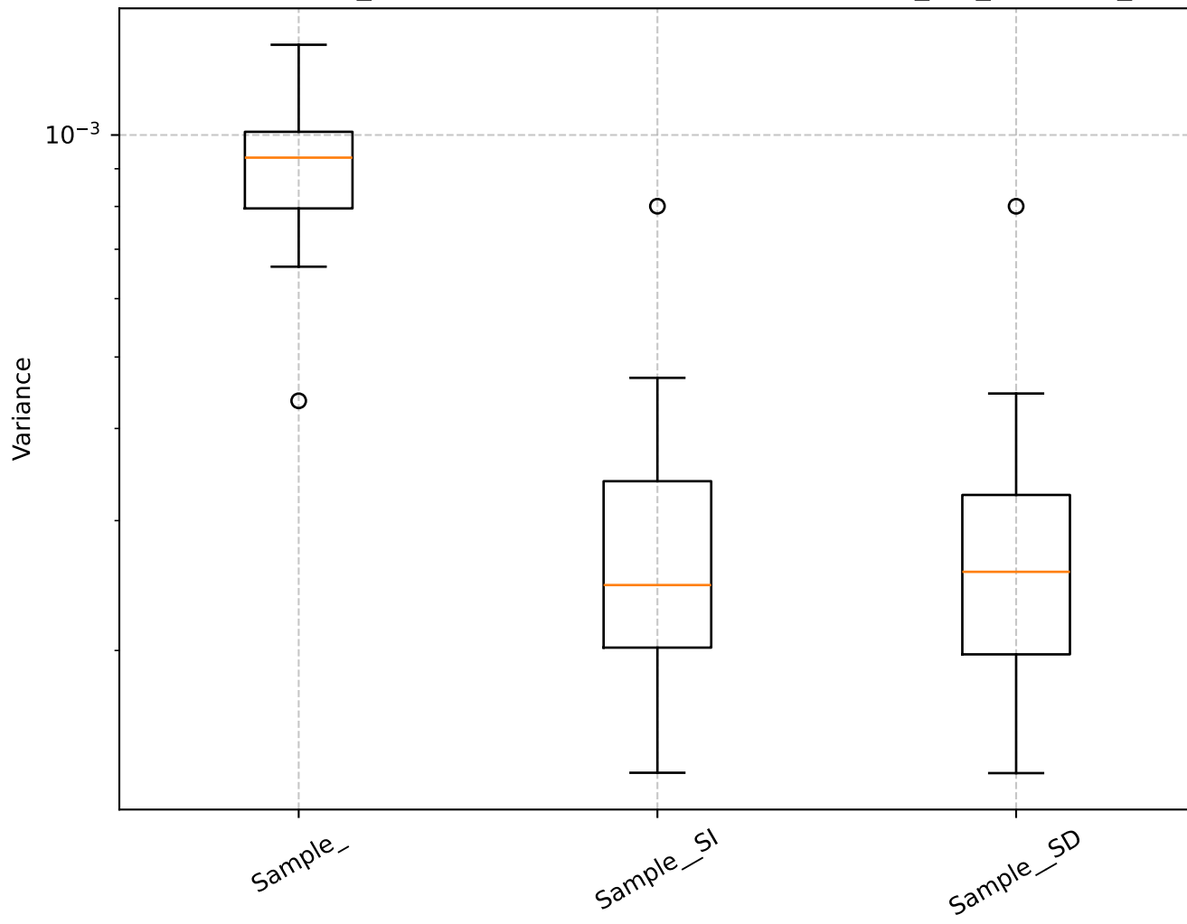
Q=0.70, len_rolling=100: Shrinkage Box Plot - min_var_, Sample_
