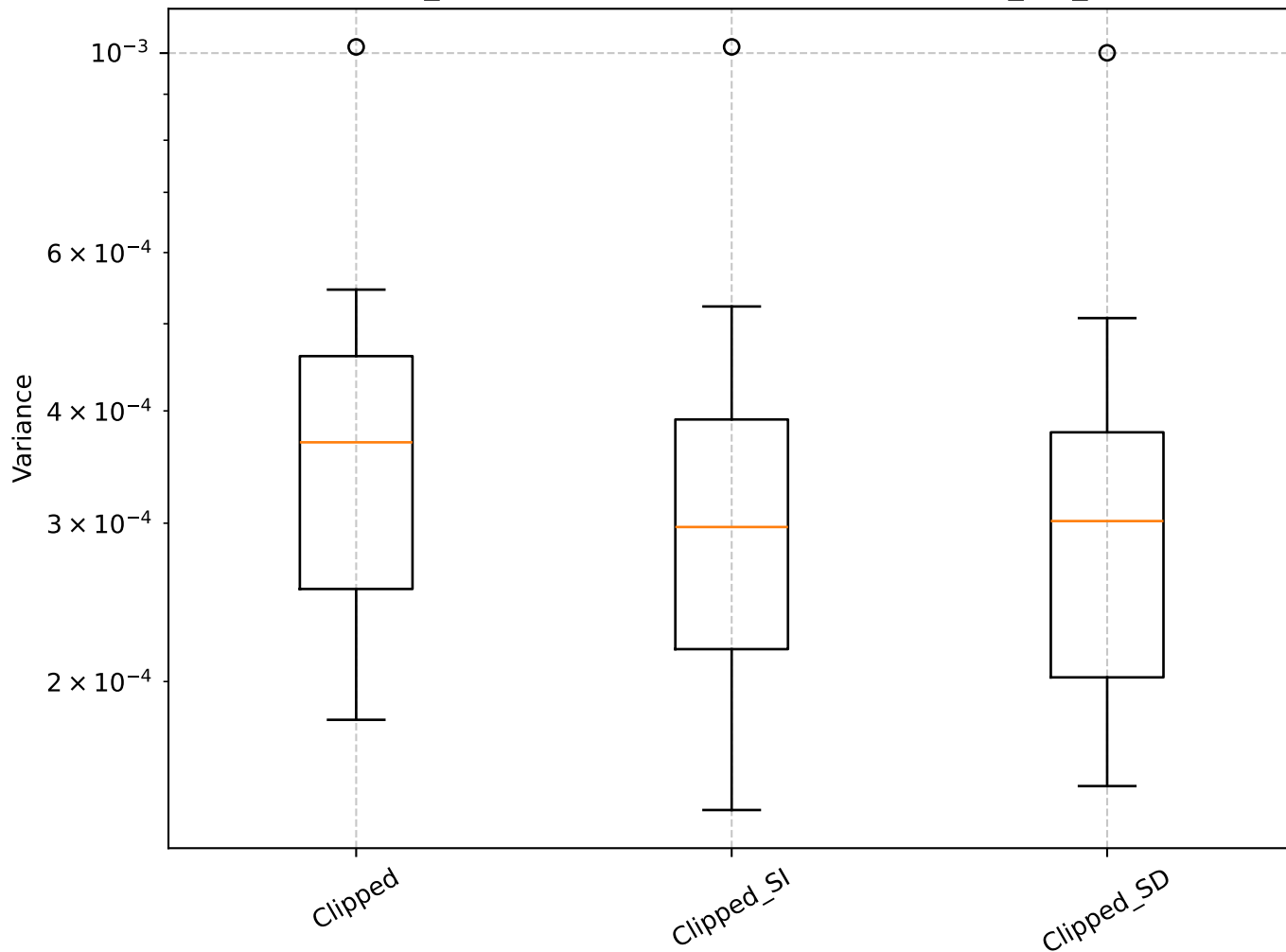
Q=0.71, len_rolling=100: Shrinkage Box Plot - min_var_, Clipped
