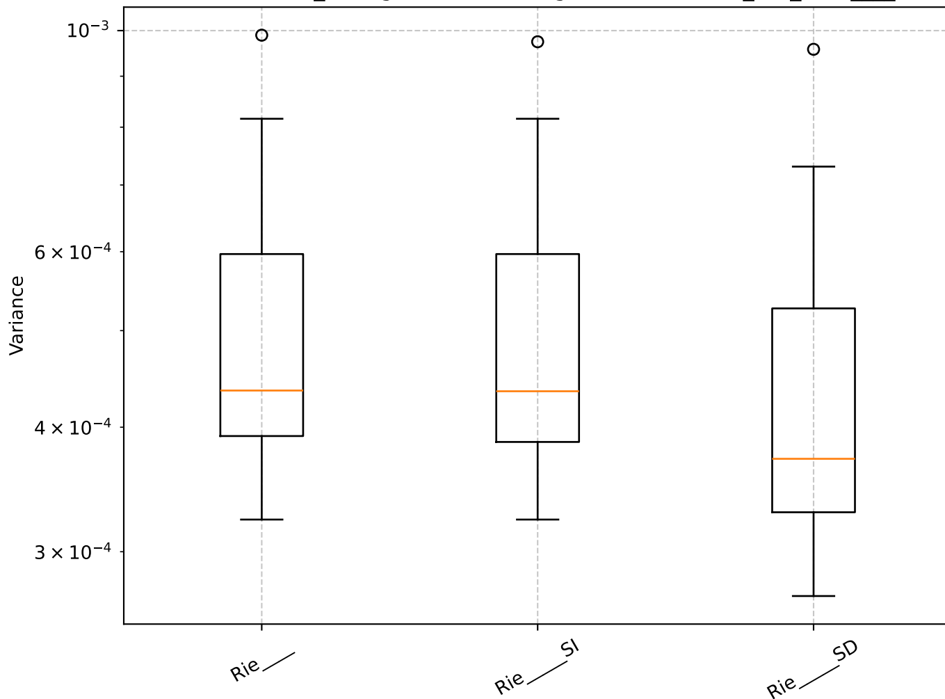
Q=0.75, len_rolling=100: Shrinkage Box Plot - min_var_, Rie____
