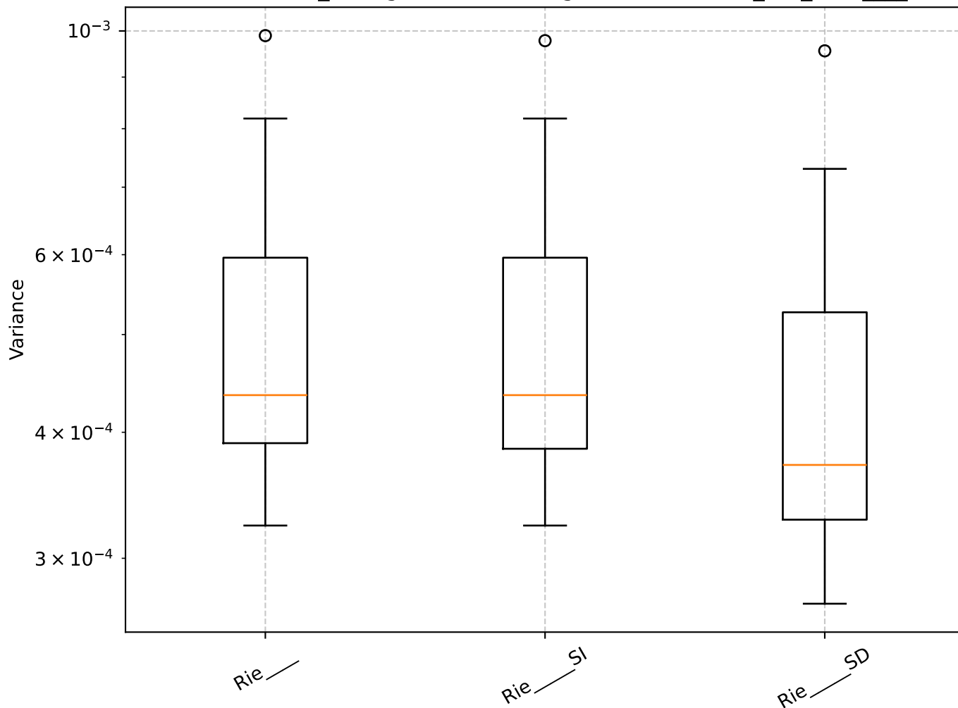
Q=0.78, len_rolling=100: Shrinkage Box Plot - min_var_, Rie____
