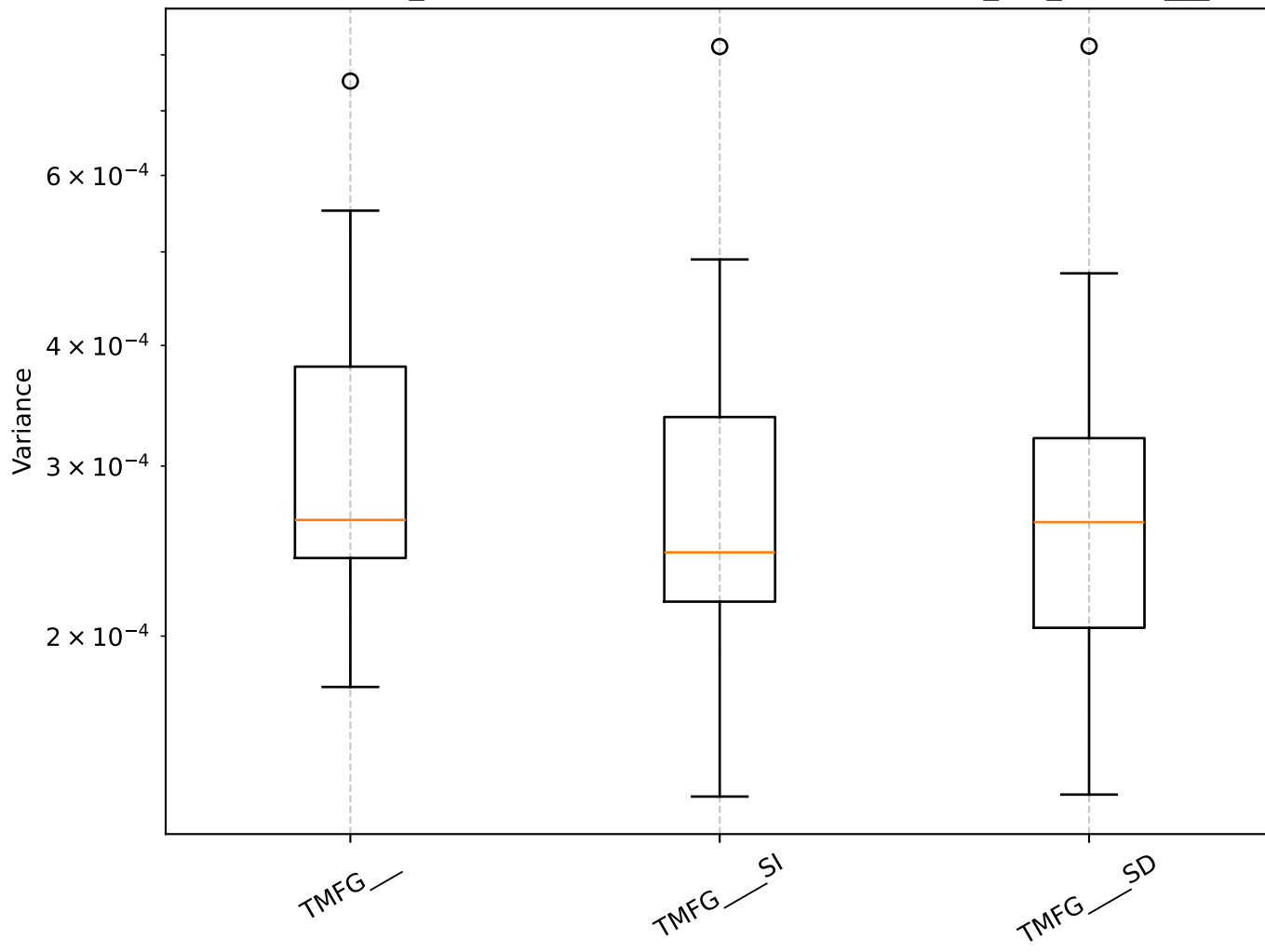
Q=0.78, len_rolling=100: Shrinkage Box Plot - min_var_, TMFG__
