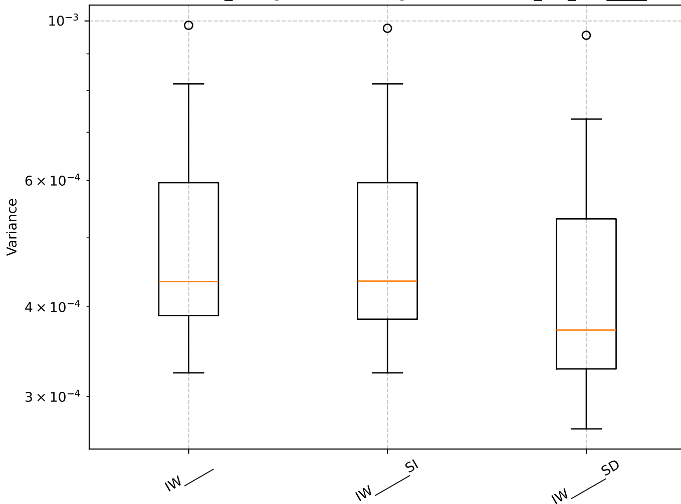
Q=0.80, len_rolling=100: Shrinkage Box Plot - min_var_, IW_____
