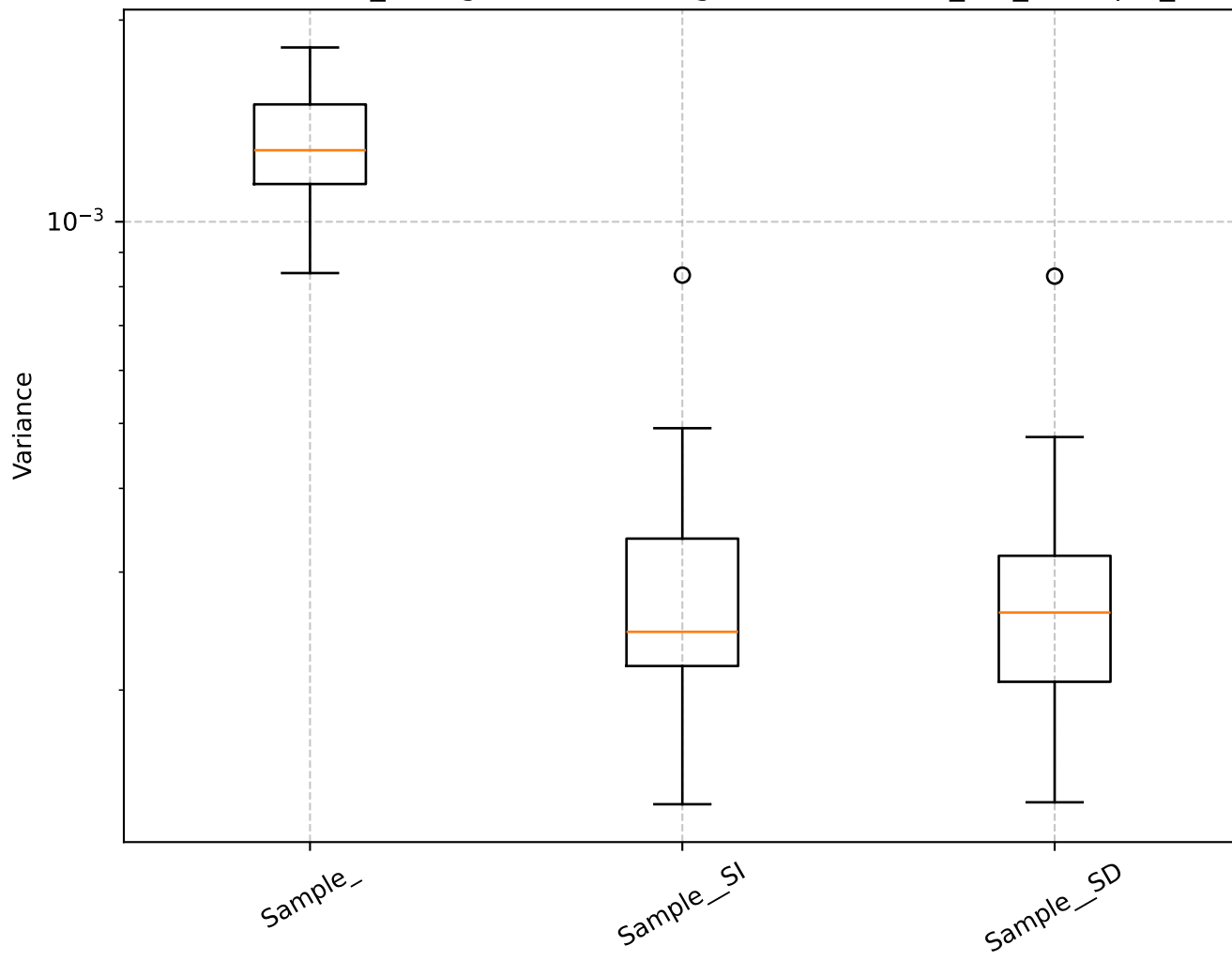
Q=0.80, len_rolling=100: Shrinkage Box Plot - min_var_, Sample_
