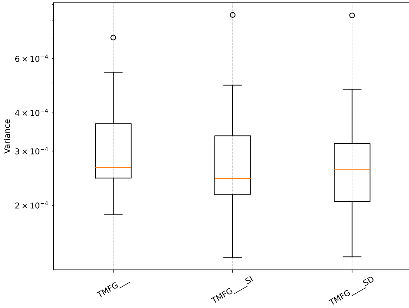
Q=0.80, len_rolling=100: Shrinkage Box Plot - min_var_, TMFG__
