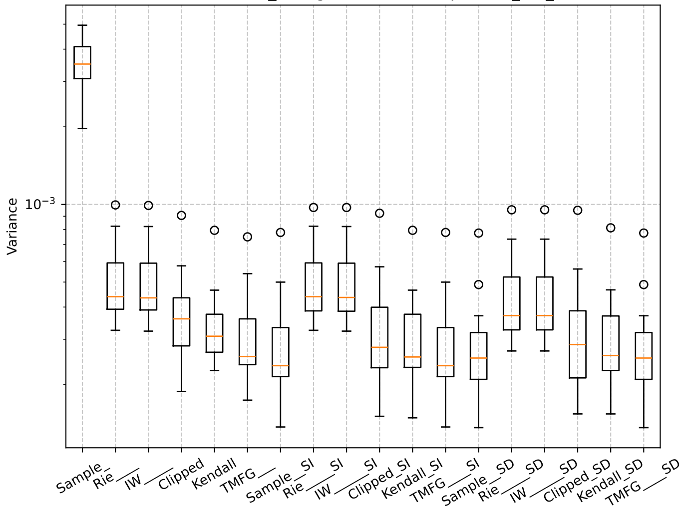
Q=0.93, len_rolling=100: Box Plot per min_var_
