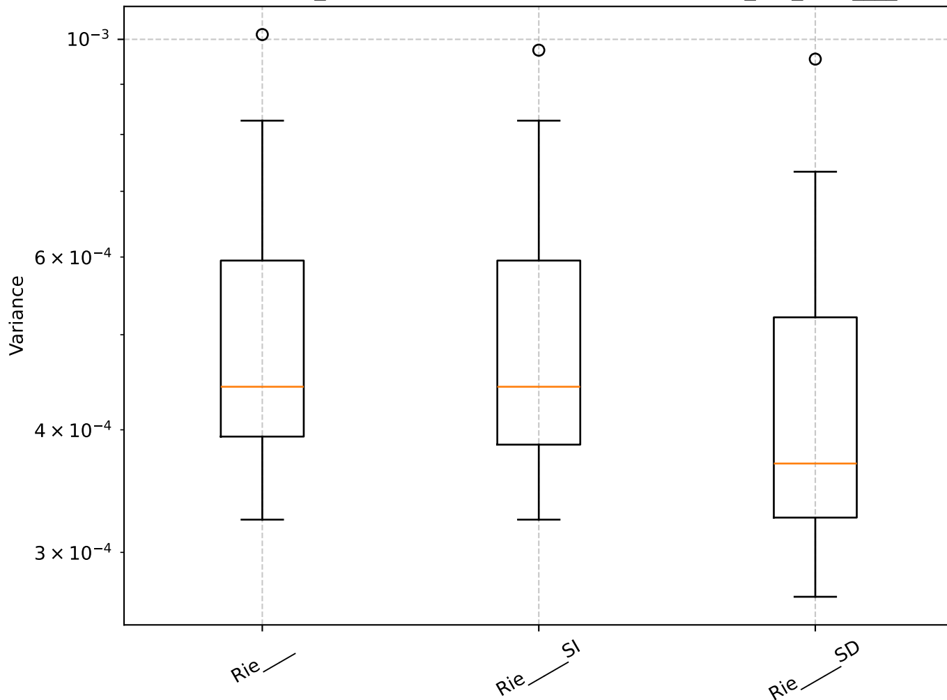
Q=0.98, len_rolling=100: Shrinkage Box Plot - min_var_, Rie__
