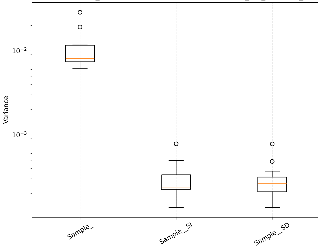
Q=0.98, len_rolling=100: Shrinkage Box Plot - min_var_, Sample_
