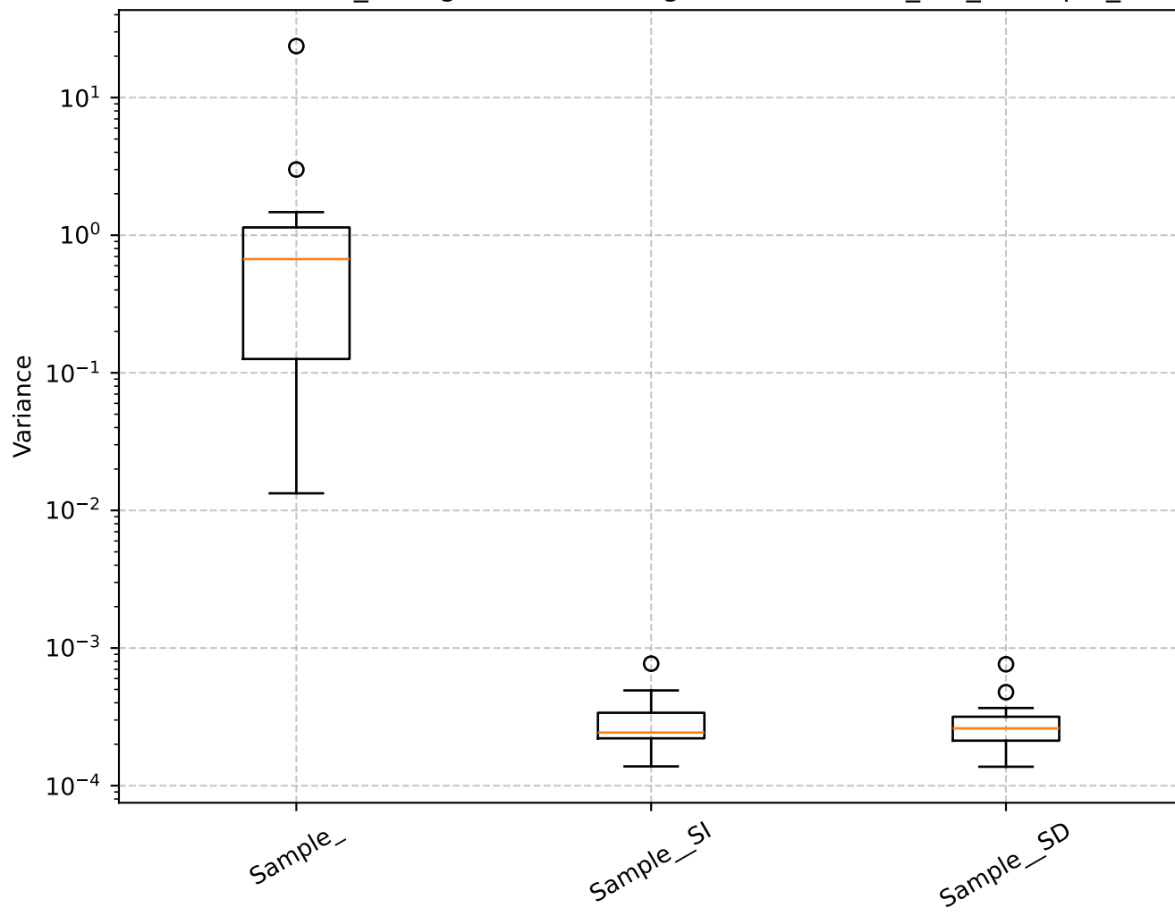
Q=1.00, len_rolling=100: Shrinkage Box Plot - min_var_, Sample_
