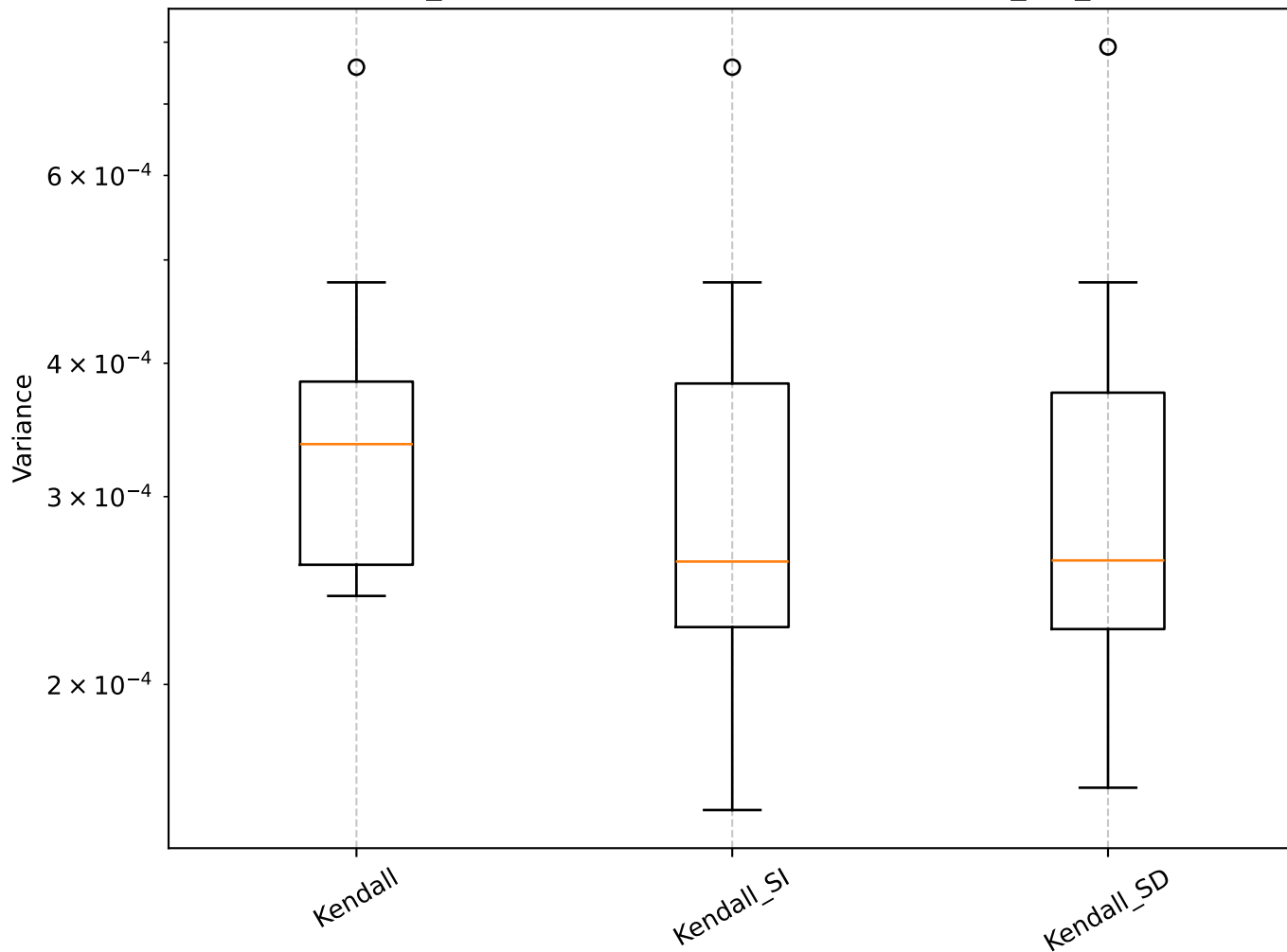
Q=1.08, len_rolling=100: Shrinkage Box Plot - min_var_, Kendall
