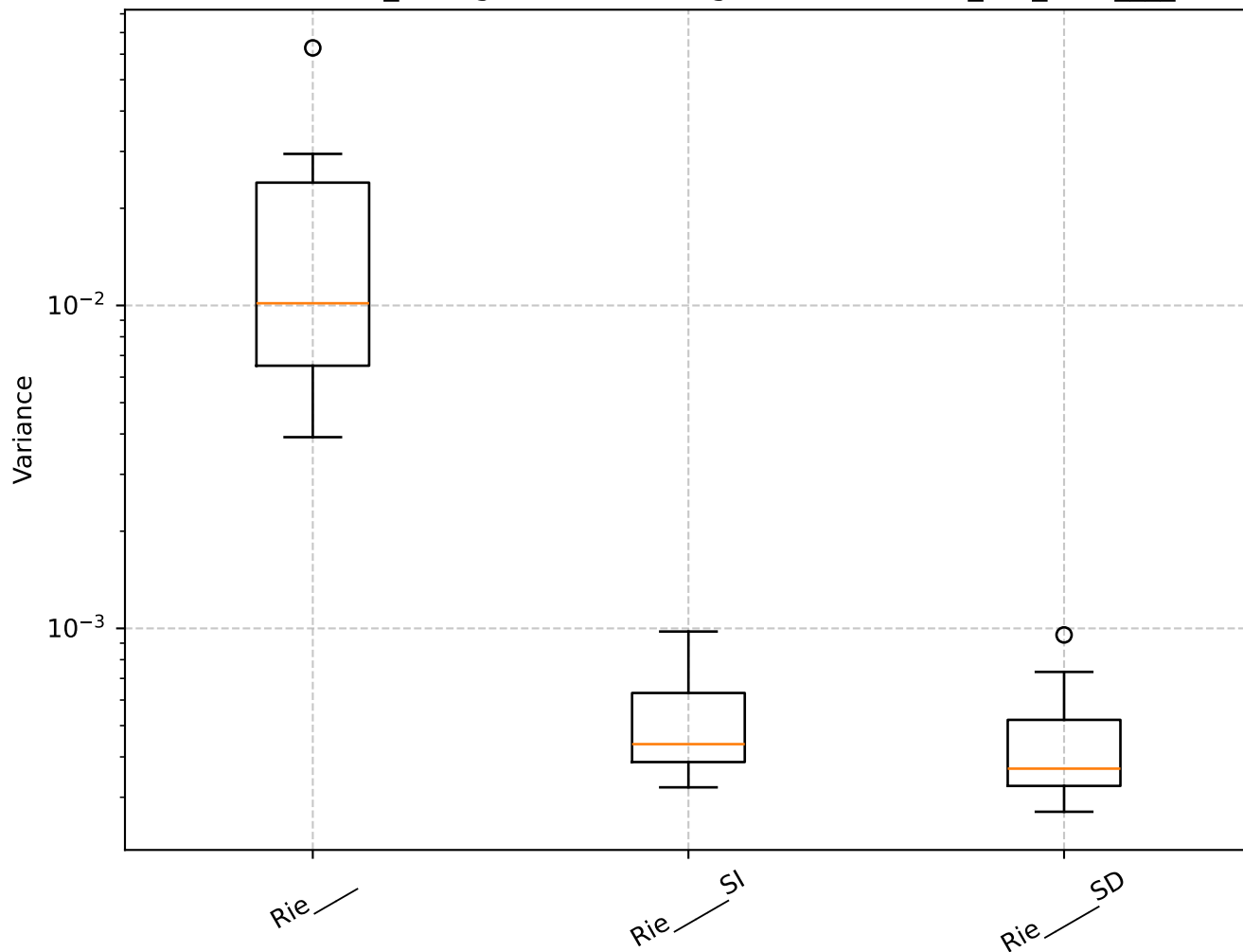
Q=1.08, len_rolling=100: Shrinkage Box Plot - min_var_, Rie____
