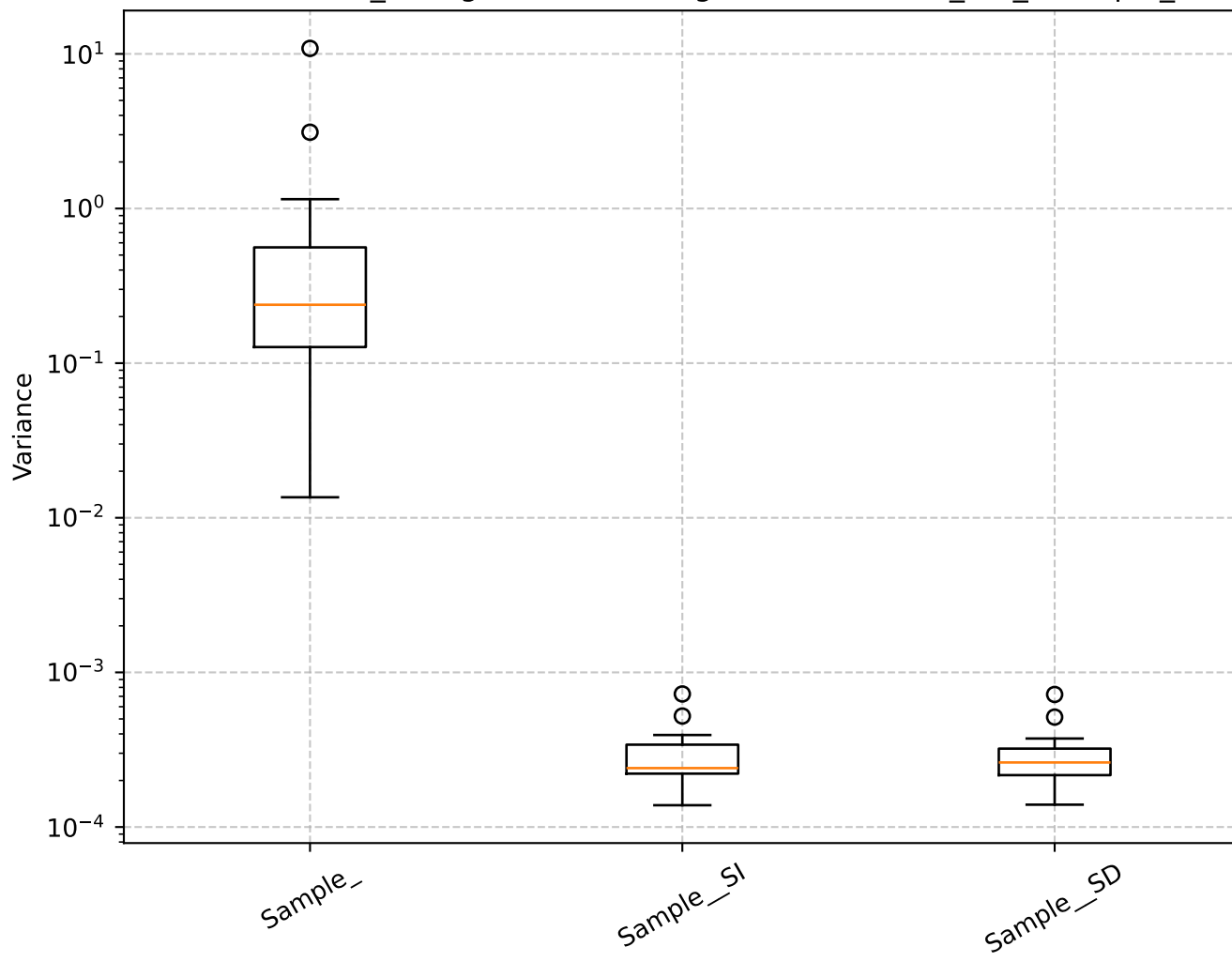
Q=1.08, len_rolling=100: Shrinkage Box Plot - min_var_, Sample_
